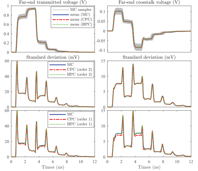
Fig. 2. Variability of the far-end transmitted (left panels) and crosstalk (right panels) voltages for a 5% parameter variation. Top panels: subset of MC samples (gray lines) and average computed from the MC samples (solid blue lines), CPC expansion (dashed red lines) and HPC expansion (dotted green lines). Central and bottom panels: standard deviation for different PC orders (the same color code is used).
