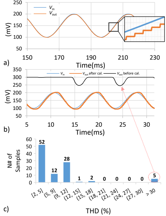
Fig. 3. a) V_{in} and V_{out} for C_{out} = 80\text{pF} , V_{amp} = 50\text{mV} and f_{in} = 30\text{Hz} . b) V_{in} , V_{out} before calibration (black) and V_{out} after calibration (red) for C_{out} = 80\text{pF} , V_{amp} = 50\text{mV} and f_{in} = 120\text{Hz} . c) 100 samples MC simulation for DB-OTA THD (%).
