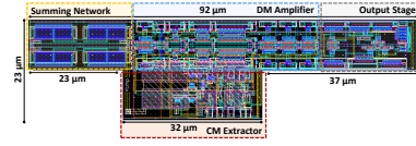
Fig. 2. DB-OTA layout. Total area of 1,426 \mu\text{m}^2 .
