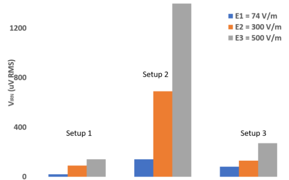
Figure 4. Measured input-referred power line interference ( \mu V_{RMS} ) for three electrode configurations and electric field intensities of 74 V/m, 300 V/m and 500 V/m respectively. When the input impedances were matched (Setup 3) the power line interference results similar to the one obtained when three big electrodes are used for the monopolar sEMG acquisition (Setup 1).
