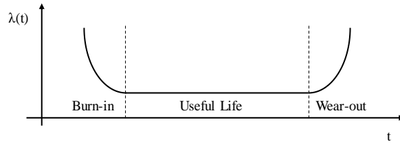
Fig. 1 Bathtub curve.
