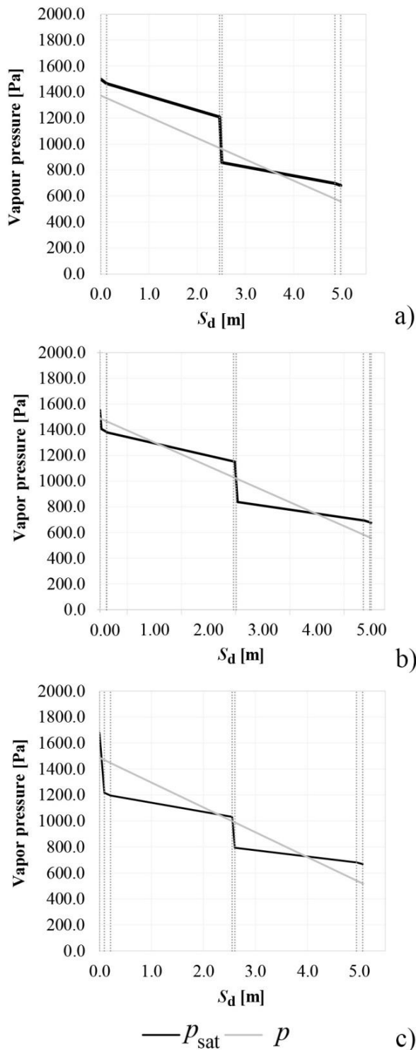
Figure 8: Vapour saturation and vapour pressure for the three different wall configurations A0 (a), A1_3 (b), A1_12 (c) for January.
