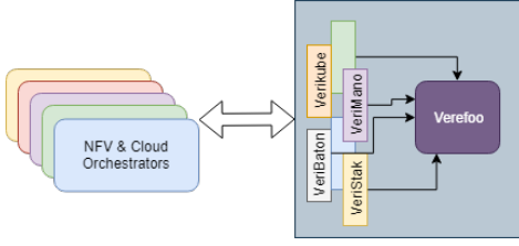
Fig. 3. Integration architecture.
