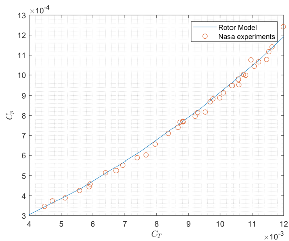
Fig. 11 XV-15 C_p - C_t trend in Hover
