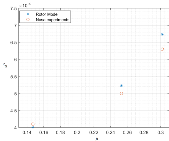
Fig. 17 UH-60 C_Q - \mu trend in forward flight
