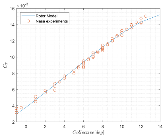
Fig. 12 XV-15 C_t - \theta trend in Hover
