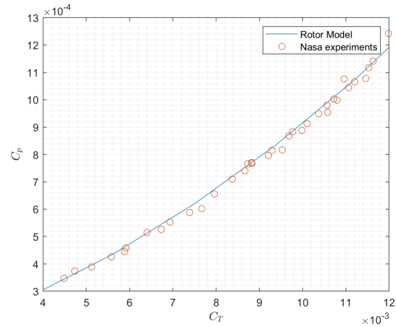
Fig. 11 XV-15 C_p - C_t trend in Hover
