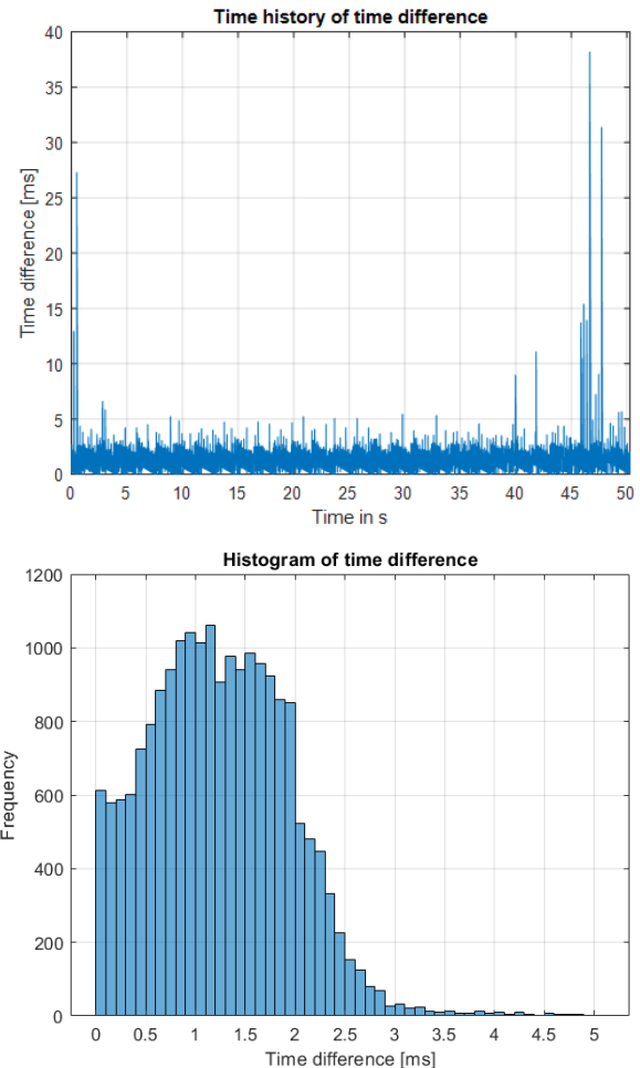
Fig. 19 Time History and histogram of the difference between simulation and computer time.
