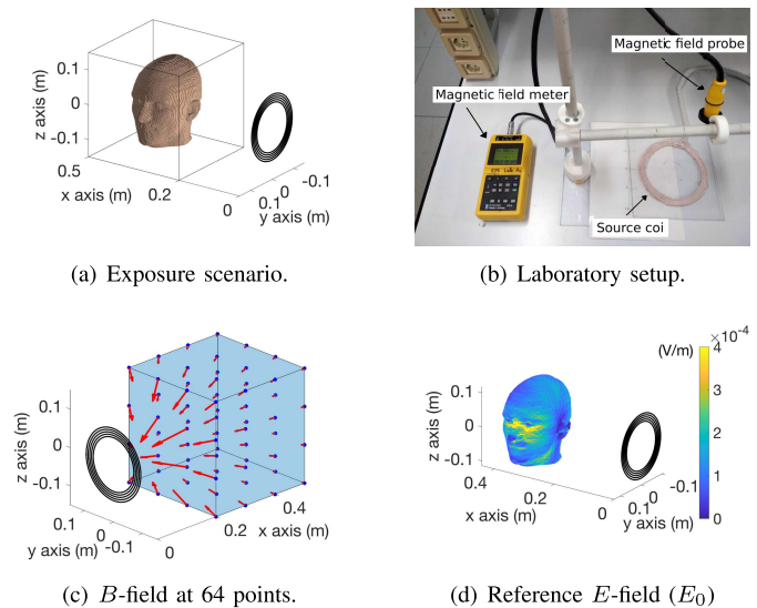
Fig. 1. (a) Exposure scenario considered in this paper. (b) Laboratory setup. (c) Measurement at discrete points with equal grid spacing along each directions. (d) Reference solution for the induced electric field.
