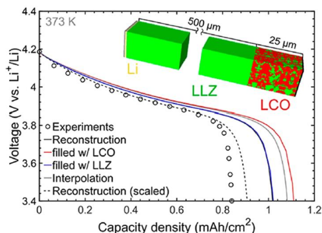
Figure 6. Simulated Li/LLZO/LCO cell based on a 3D reconstruction derived from FIB-SEM tomography (Inset). Discharge curves at 100 °C from experimental measurement (open circles) and from simulated data for as reconstructed (black) and void-filled mixed cathode (red = LCO, gray = mixed, blue = LLZ). Reproduced, adapted and reprinted with permission from Ref 38.
