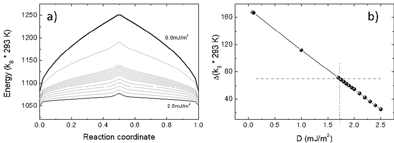
FIG. 2. (a) Evolution of the MEP with the D value in the range 0.0–2.5 \text{mJ/m}^2 for a 100 nm wide square dot. (b) Variation of the thermal stability factor \Delta with D estimated at room temperature. The gray dotted line indicates the 70k_B T threshold.
