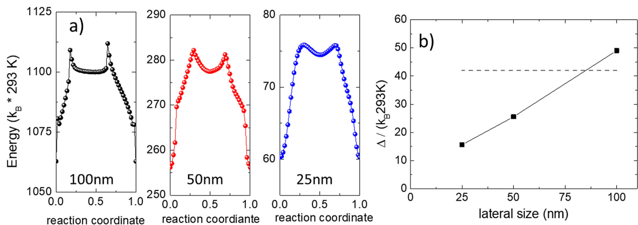
FIG. 3. (a) MEP profile for 100 nm (black), 50 nm (red), and 25 nm (blue) lateral size dots with D = 2 \text{ mJ/m}^2 . (b) Thermal stability factor \Delta as a function of the lateral size L estimated at room temperature. The gray dotted line indicates the 42k_B T threshold.
