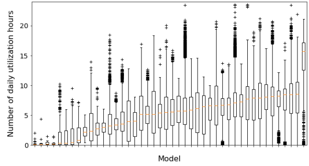
(b) Boxplots of number of daily utilization hours for different models of a single vehicle type (all refuse compactors)
