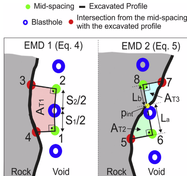
Fig. 5. Calculation of the Excavated Mean Distance.
