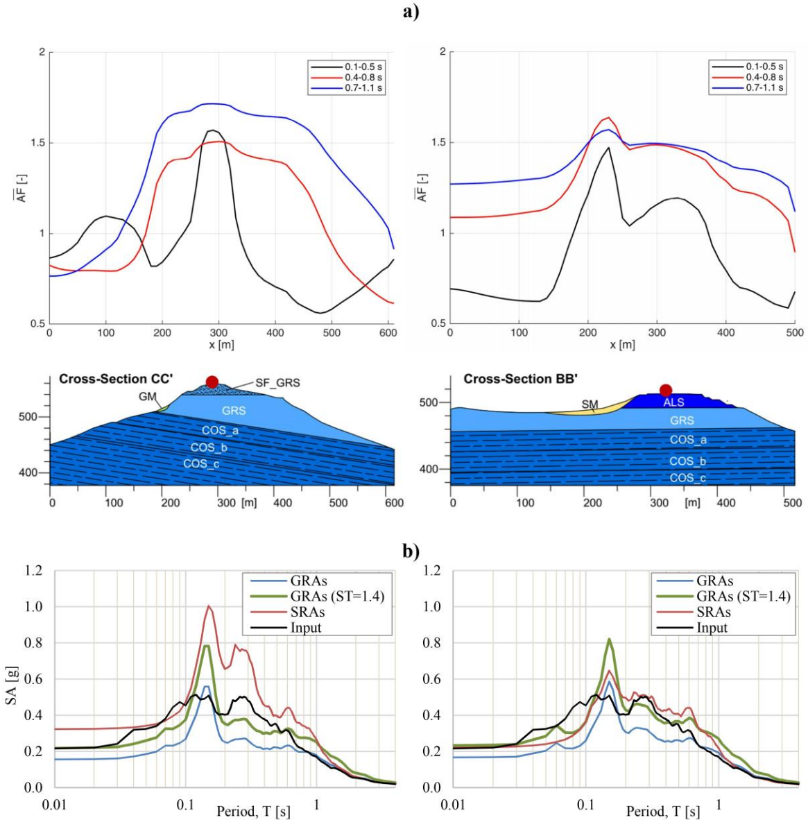
Figure 6 Results for the Montedinove site in terms of a) \overline{AF} s and b) SA s from GRAs, SRAs and GRAs with an aggravation topographic factor (as defined by NTC18) of 1.4 (modified from Pagliaroli et al., 2019).
