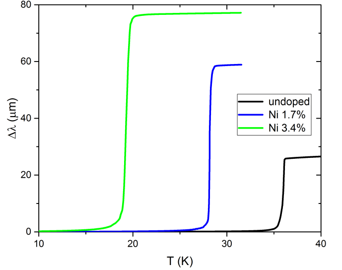
FIG. 1. Temperature dependence of \Delta\lambda_{L,ab} for all doping levels measured with the TDR technique. The critical temperatures reported in Tab. I correspond to the maximum of the temperature derivative of these curves. The good quality and low disorder level of the samples is testified by the narrow transitions.
