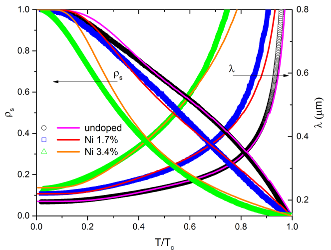
FIG. 4. Experimental \rho_s and \Delta\lambda_L vs T curves for all doping levels (black circles for the undoped sample, blue squares for 1.7% Ni and green triangles for 3.4%) compared to the results of the Eliashberg calculations shown as solid lines.
