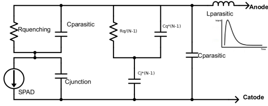
Fig. 4: SiPM electrical model with the parasitic inductance due to interconnections
