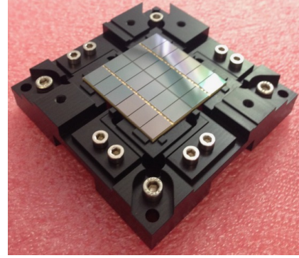
Fig. 1: A 24 cm 2 SiPM tile developed by the Darkside Collaboration.
