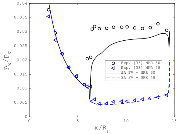
Fig. 4 Wall pressure distribution in dual-bell nozzle.
