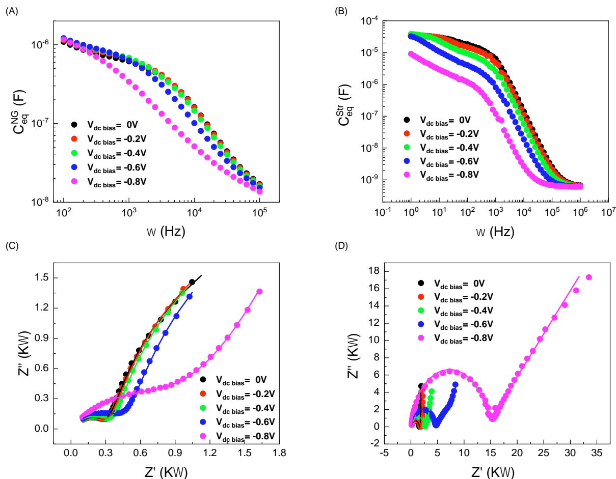
Figure 4. Equivalent capacitance C_{eq}(=1/(2\pi fZ'')) as a function of the ac signal frequency ( \pm 10 mV) in the case of (A) a Nanogap-OECT and (B) a stripe-like OECT, recorded in presence of the superimposed dc biases; Nyquist plots in presence of negative dc biases for (C) a Nanogap-OECT and (D) a stripe-like OECT; fitting curves (as line plots) upon equivalent circuit analysis are reported too. For all the reported measurements, V_{dc\ bias}=0 (black symbols-lines), V_{dc\ bias}=-0.2 (red symbols-lines), V_{dc\ bias}=-0.4 (green symbols-lines), V_{dc\ bias}=-0.6 (blue symbols-lines) and V_{dc\ bias}=-0.8 V (magenta symbols-lines).
