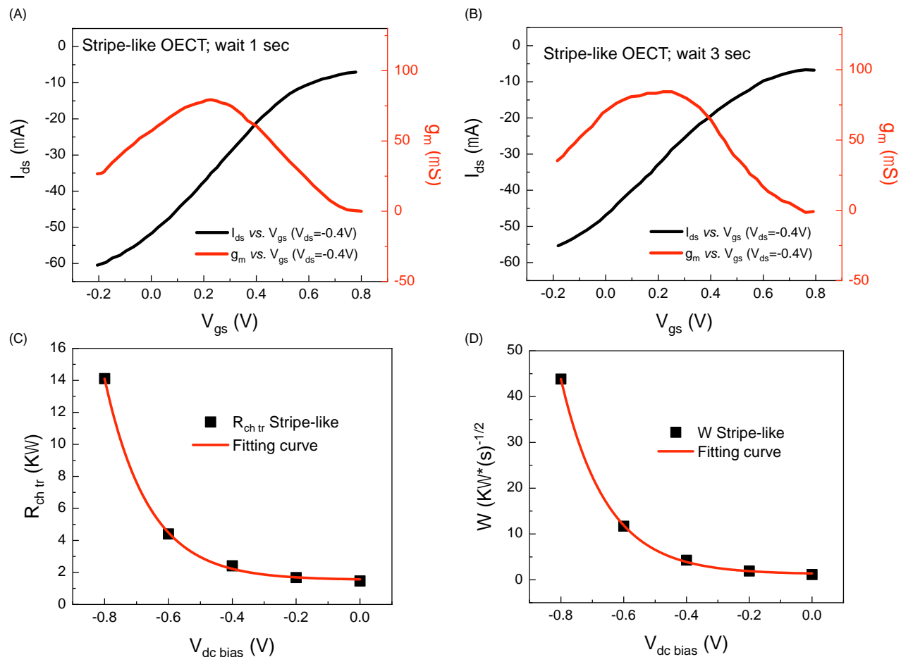
Figure 7. Transfer curves (black line) and transconductance (red line) as a function of V_{gs} for a stripe-like OECT at t_{scan} = 1 s (A) and 3 s (B); (C) charge transfer resistance ( R_{ch-tr} ) and (D) Warburg coefficient ( W ) reported in Table 2 as a function of V_{dc} bias (fitting curves in red) for a stripe-like OECT.
