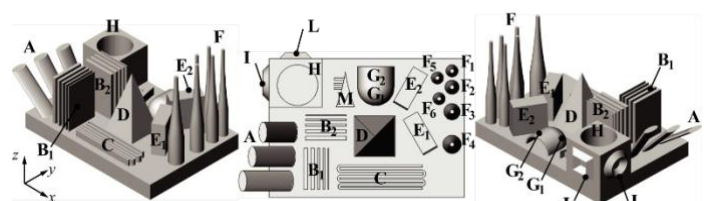
Fig. 2. Reference part.
