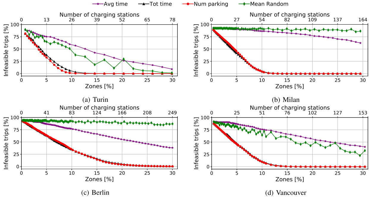
Fig. 5. Percentage of infeasible trips as function of charging station number for the Free Floating return policy. Placing charging stations where cars are frequently parked (Tot time and Num parking) is much better than where cars stay parked for long time (Avg time).
