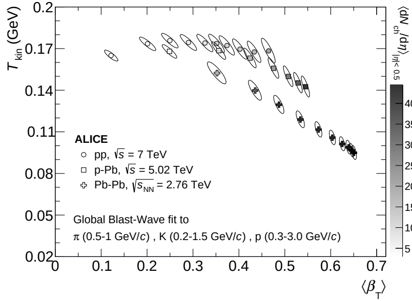
Fig. 14: Kinematic freeze-out temperature parameter T_{kin} versus average expansion velocity \langle \beta_T \rangle from a simultaneous BG-BW fit to \pi , K and p spectra measured in pp, p-Pb and Pb-Pb collisions. The shade of the datapoints indicates the corresponding average charged-particle multiplicity density.
