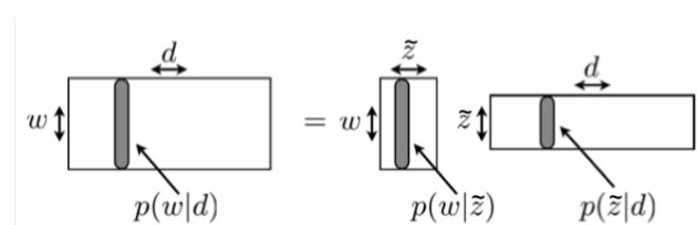
Fig. 3. Reverse Generative Process.
