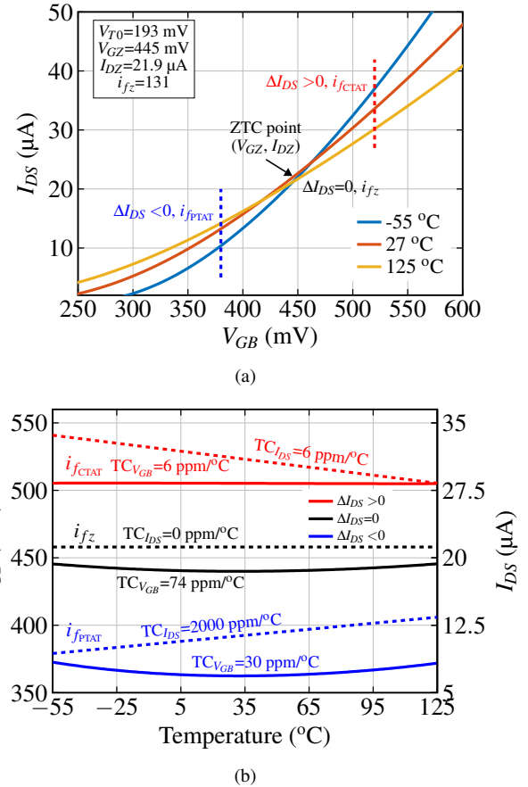
Fig. 1. (a) ZTC condition for a standard NMOS transistor in a 0.13- \mu\text{m} CMOS process. (b) In solid line, V_{GB}(T, \Delta I_{DS} = I_{DS} - I_{DZ}) with the right amount of thermal drift TC_{I_{DS}} applied into the MOS transistor. In dashed line, the bias currents with the needed thermal drift TC_{I_{DS}} .
