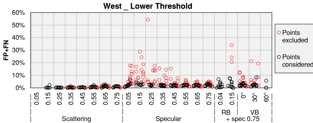
Figure 39. Errors after the data screening relative to the estimation of the daylight glare comfort classes using the E_v lower threshold in the west orientation. Red markers represent the points not considered.
