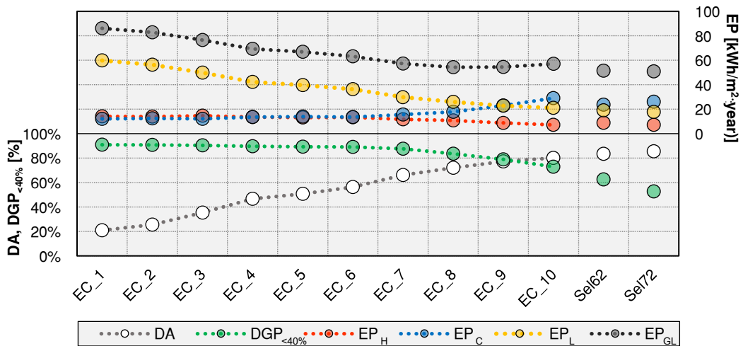
Figure 27. Annual results relative to energy performance (upper chart) and visual comfort (lower chart) for the two selective glazings and the 10 states of the Electrochromic glazing.
