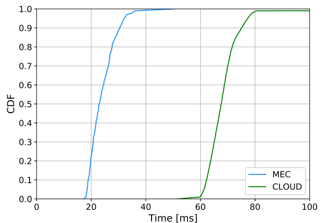
Fig. 10: CDF of the network latencies in the MEC and in the cloud experiments
