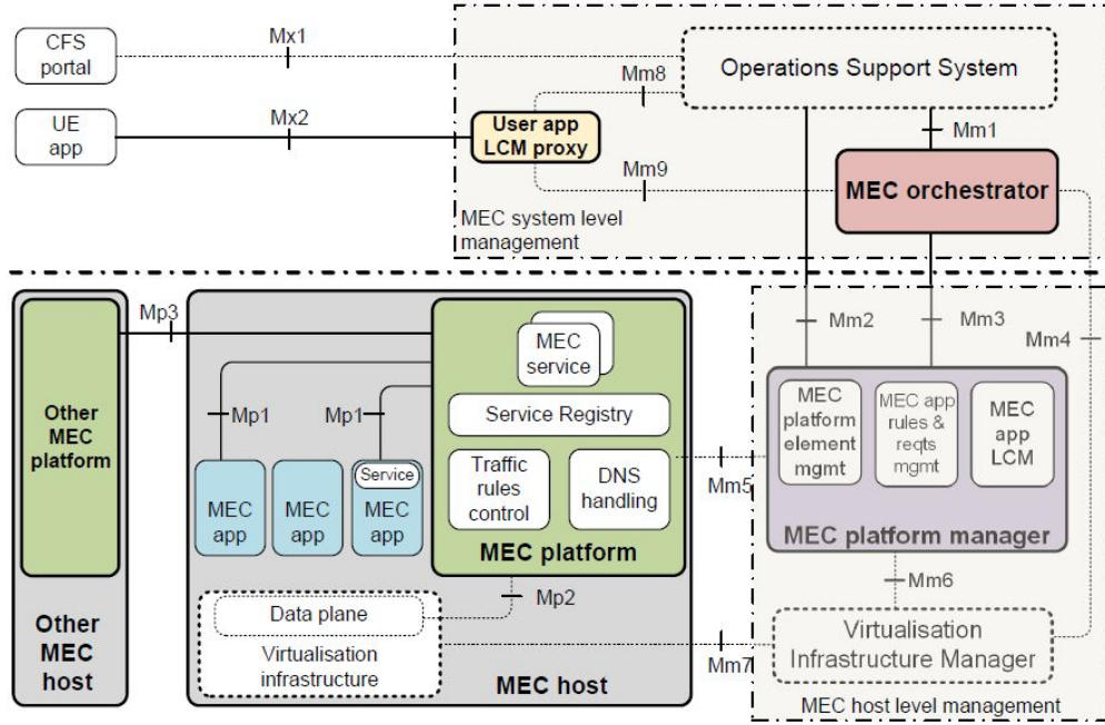
Fig. 1: ETSI MEC architecture [1]
