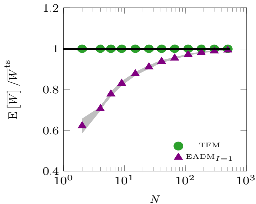
Fig. 7 Accuracy of the EADM_{I=1} and the TFM in estimating the total number of temporal links in the overall time series. A perfect identification should yield a ratio between E[\bar{W}] and \bar{W}^{ts} of one (black solid line). In these simulations, we use our artificial network where no backbone is present ( \delta = \lambda = 0 ) and activities are constant in time ( T = 5,000 , I = 1 , \langle \tau(\Delta) \rangle = T/I = 5000 , a_{\min} = \lfloor \sqrt{\langle \tau(\Delta) \rangle} \rfloor^{-1} , and p = 0 ). Markers indicates the average of 10^2 independent simulations, 95% confidence interval is displayed in gray.
