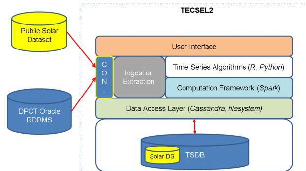
Fig. 2. TECSEL2 High Level Architecture
