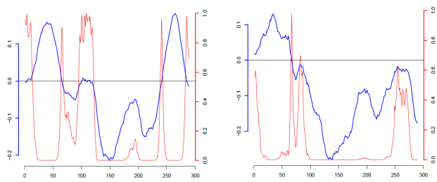
Fig. 5. Partial correlation between OMNI variables and AIM (mag<13) variables on May 11-15,2015. OMNI proton flux vs. AIM flux; OMNI proton flux vs. AIM background.
