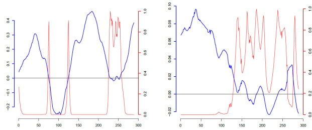
Fig. 4. Partial correlation between OMNI variables and AIM variables on Dec.12-25,2014. OMNI proton density vs. AIM (mag<13) flux; OMNI flow pressure vs. AIM (15<mag<16). background
