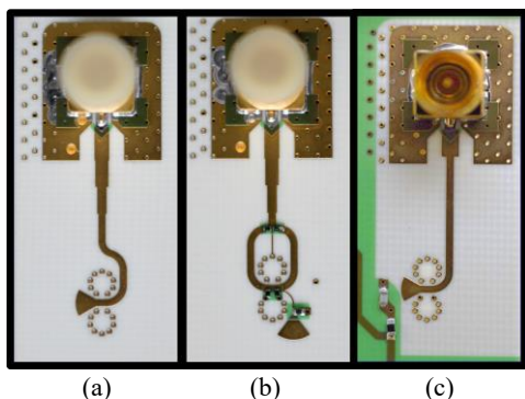
Fig. 9. Manufactured and measured phase shifters, including the SMP connector; (a) 0^\circ fixed phase shifter, array side; (b) 0^\circ/180^\circ reconfigurable phase shifter, array side; (c) 0^\circ fixed and 0^\circ/180^\circ reconfigurable phase shifter, Rotman lens side (identical for the two types of phase shifters).
