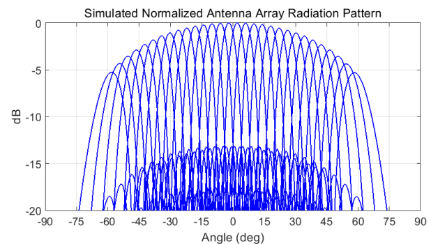
Fig. 5. Simulated normalized antenna array radiation pattern at 24 GHz with ideal excitation, scanning at \pm 60^\circ .
