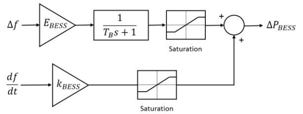
Fig. 2. Dynamic model of a BESS
