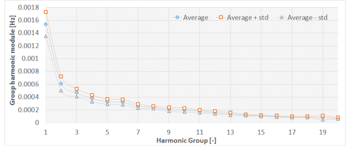
Figure 2. Real Data Module Harmonics Groups
