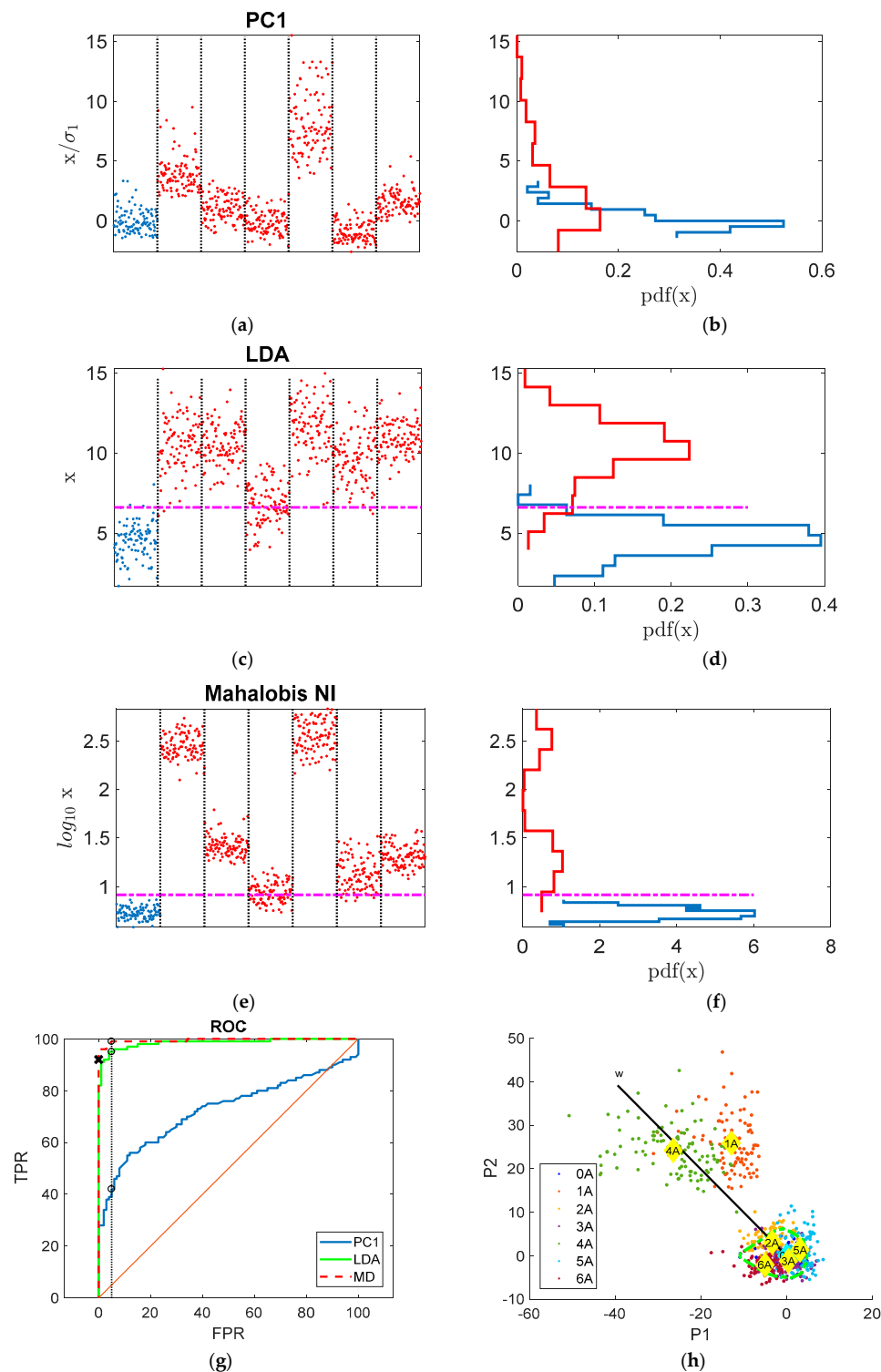
Figure 15. Results for condition 3 (90 Hz, 1400 N) alone ( a,c,e ) the 3 different dimensionality reductions; ( b,d,f ) the corresponding empirical pdf for the healthy condition (blue) and for the 6 damage conditions (red). The x axis represents the 100 observations for each of the different damage conditions (ordered from 0A to 6A) which are separated by the black dotted lines. ( g ) ROC curves for the three 1-D reductions. The 5% significance threshold values are highlighted with the black circles; the black x denotes the position of the NI threshold computed according to the MC repetition introduced in Section 2.4.1—in magenta in ( h ) The 2-D PCA visualization of the dataset (condition 12) and the LDA direction w .
