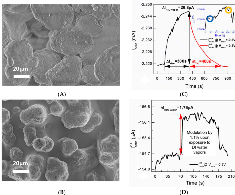
Figure 2. SEM images of (A) the sintered polyamide (1500×) and (B) the same coated by a poly(3,4-ethylenedioxythiophene):polystyrene sulfonate (PEDOT:PSS) film (1000×); (C) real-time I_{sens} change produced by water vaporization at a distance of 1 mm (black branch) and reversibility check (restoring of the initial I_{sens} value upon removal of the water reservoir, red branch). The inset shows the device behavior upon exposure to an empty reservoir and removal of the same reservoir (20 s lasting effects on the recorded current upon reservoir exposure and removal are indicated by the blue-circled and orange-circled regions, respectively);
