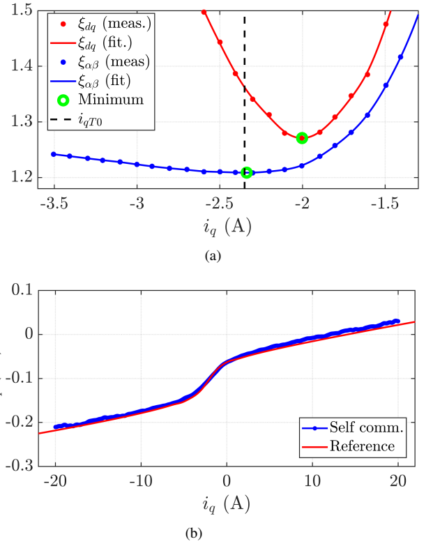
Fig. 10. (a) Evaluated saliency along q axis with (blue) or without (red) considering ellipse rotation. Black dashed line: reference i_{qT0} . (b) Final \lambda_q(i_q) characteristic obtained from stand-still self-commissioning.
