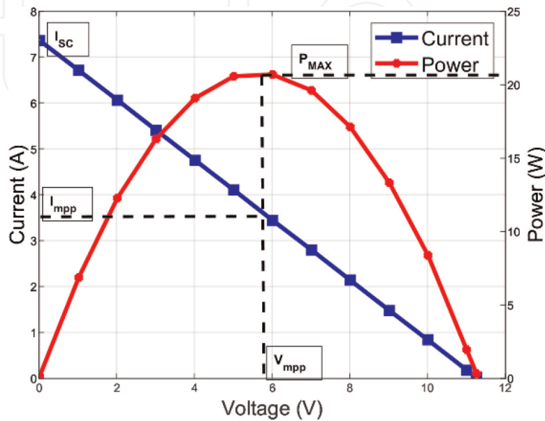
Figure 5. Current-voltage and power-voltage characteristics.
