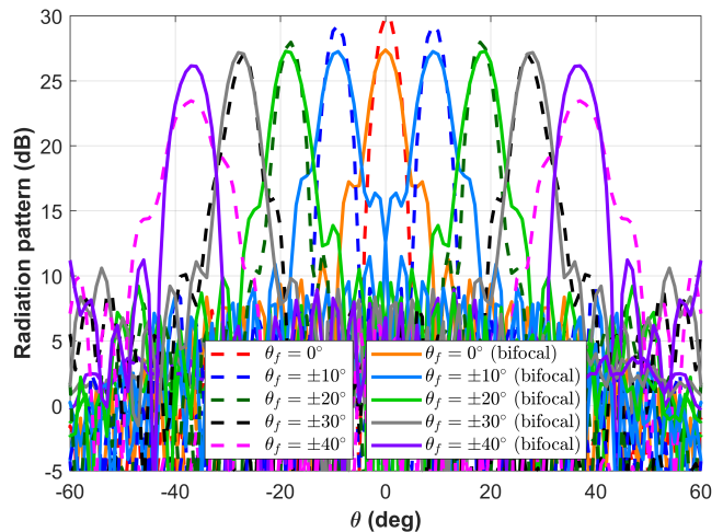
Fig. 2: Comparison of the radiation patterns (E-plane) at 30 GHz for different scanning angles.
