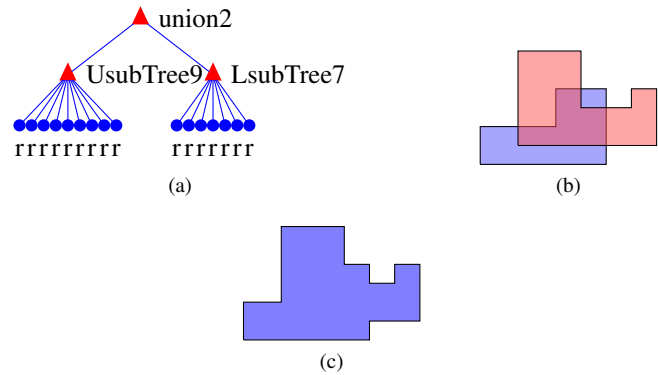
Fig. 3. An illustration of how union2 sub-tree work
