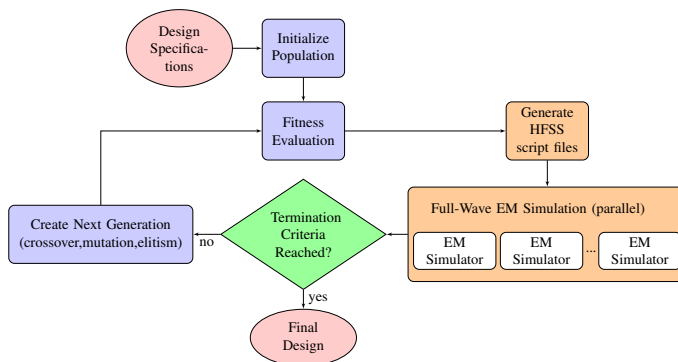
Fig. 1. Flow chart of GP software
