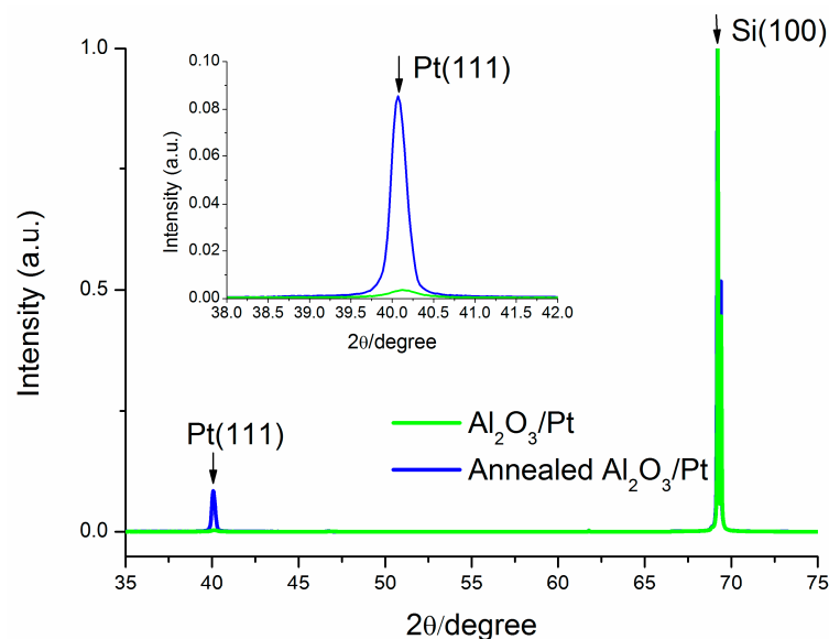
Figure 4. X-ray diffraction (XRD) patterns of \text{Al}_2\text{O}_3/\text{Pt} samples, before and after annealing at 1000 °C. Annealed sample shows the amplification of Pt(111) phase which is suitable for graphene growth. The inset shows a magnification of the Pt(111) phase.
