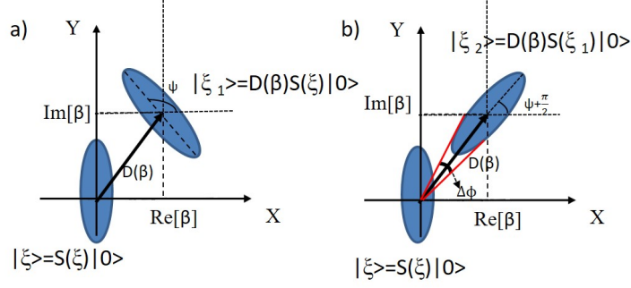
Figure 1.4: a) Amplitude squeezed b) Phase squeezed where \xi_1 = \xi e^{i\frac{\pi}{2}}
