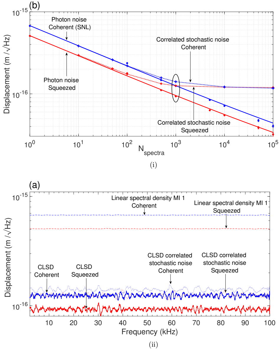
Figure 5.11: (i) The figure above presents the Displacement sensitivity ( \frac{m}{\sqrt{Hz}} ) as function of Number of Spectra. (ii) The figure above corresponds to the Displacement Sensitivity (evaluated at N_{spectra} = 1000 and PSDs of the first interferometer).
