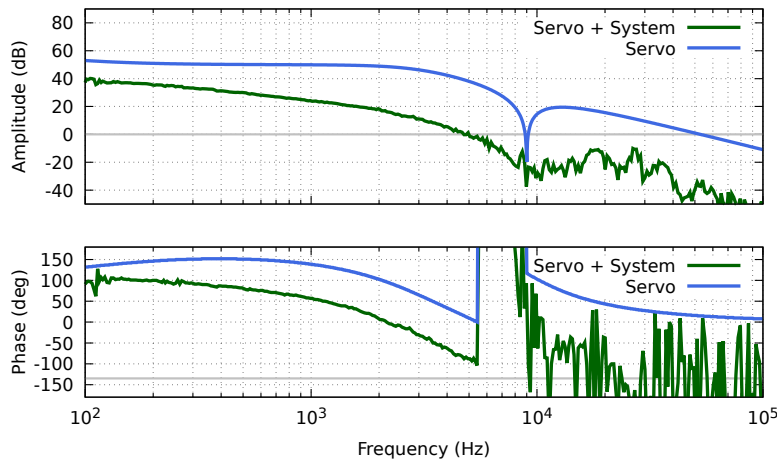
Figure B.6: Simulation on the measured transfer function. The servo was designed with integrator frequency 1.6 KHz and proportionality factor of 60dB. The expected unity gain frequency was about 3kHz.
