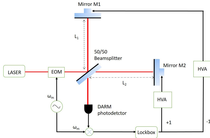
(i) Schnupp locking technique scheme of the interferometer
