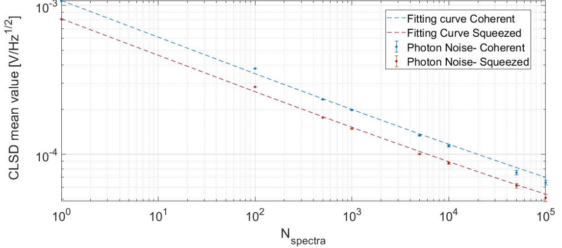
Figure 5.9: The Cross linear spectral density plotted as a function of N_{spectra} . It can be seen that in the case of no noise injected the CLSD scales as N_{spectra}^{-\frac{1}{4}} . The blue trace corresponds to coherent states while the red trace corresponds to squeezed light injection.
