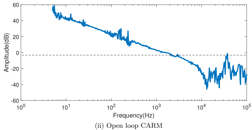
Figure B.7: (i) Open loop measurement for the DARM, (ii) Open loop measurement for CARM. The unity gain frequency obtained was around 1.3 kHz
