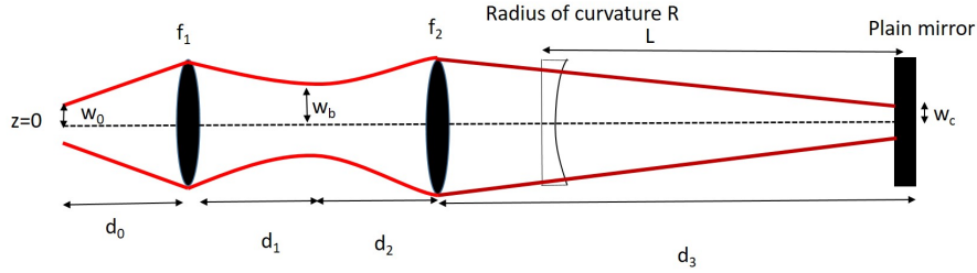
Figure A.2: Optical modematching for Fabry P erot cavity
