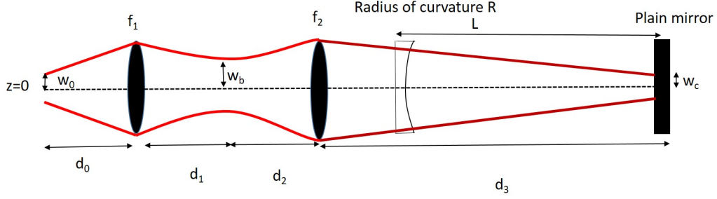
Figure 2.7: Lenses with focal lengths f_1 and f_2 are placed to mode match the input beam to the cavity.
