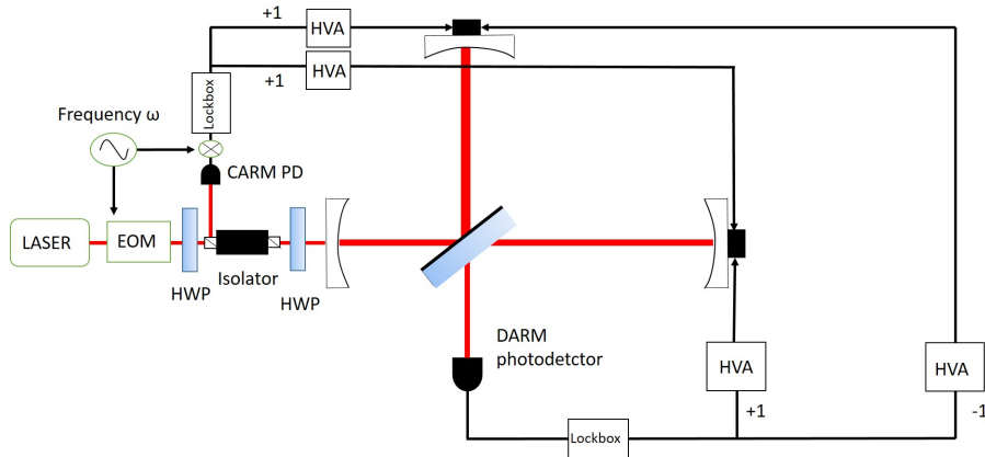
Figure 2.20: DC locking: The DARM is locked using the DC locking technique and the CARM is locked using the Pound -Drever-Hall technique. The DARM output signal is directly sent differentially to end mirrors (i.e by phase shift of \pi ) while the CARM error signal equally to end mirrors. The error signal of the CARM is obtained by demodulating the PD output at frequency \omega and is locked to the zero which corresponds to the resonance of the cavity as mentioned in section 2.2.1. PD: Photodiode; HWP :Half wave plate; HVA: High voltage Amplifier; EOM:Electro optic Modulator.
