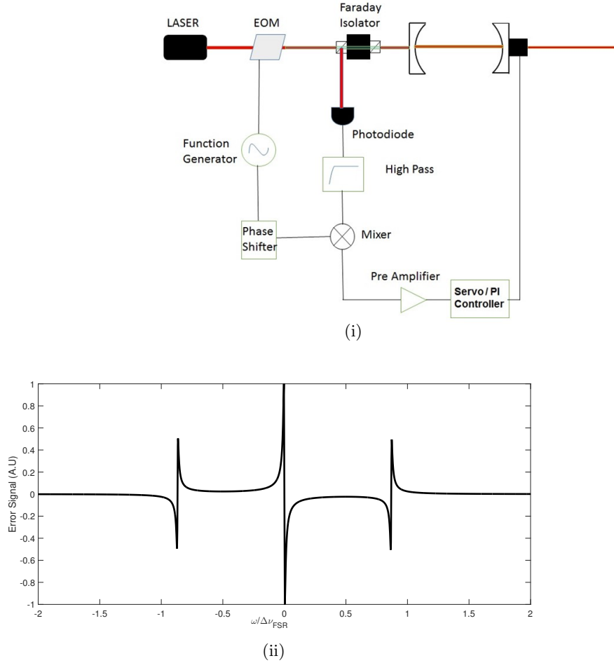
Figure 2.5: (i) The Feedback Experimental scheme. The EOM produces sidebands and the error signal is generated by demodulating the reflection signal and (ii) The Pound-Drever-Hall error signal of the cavity
