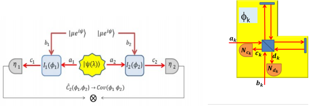
Figure 1.12: (i)The figure above represents the experimental scheme. Each interferometer is represented by I_k with coherent states injected in b_k and quantum states in a_k of the interferometers where k=1,2 . (ii) The figure represents the Michelson interferometer with quantum light injected in port a_k .
