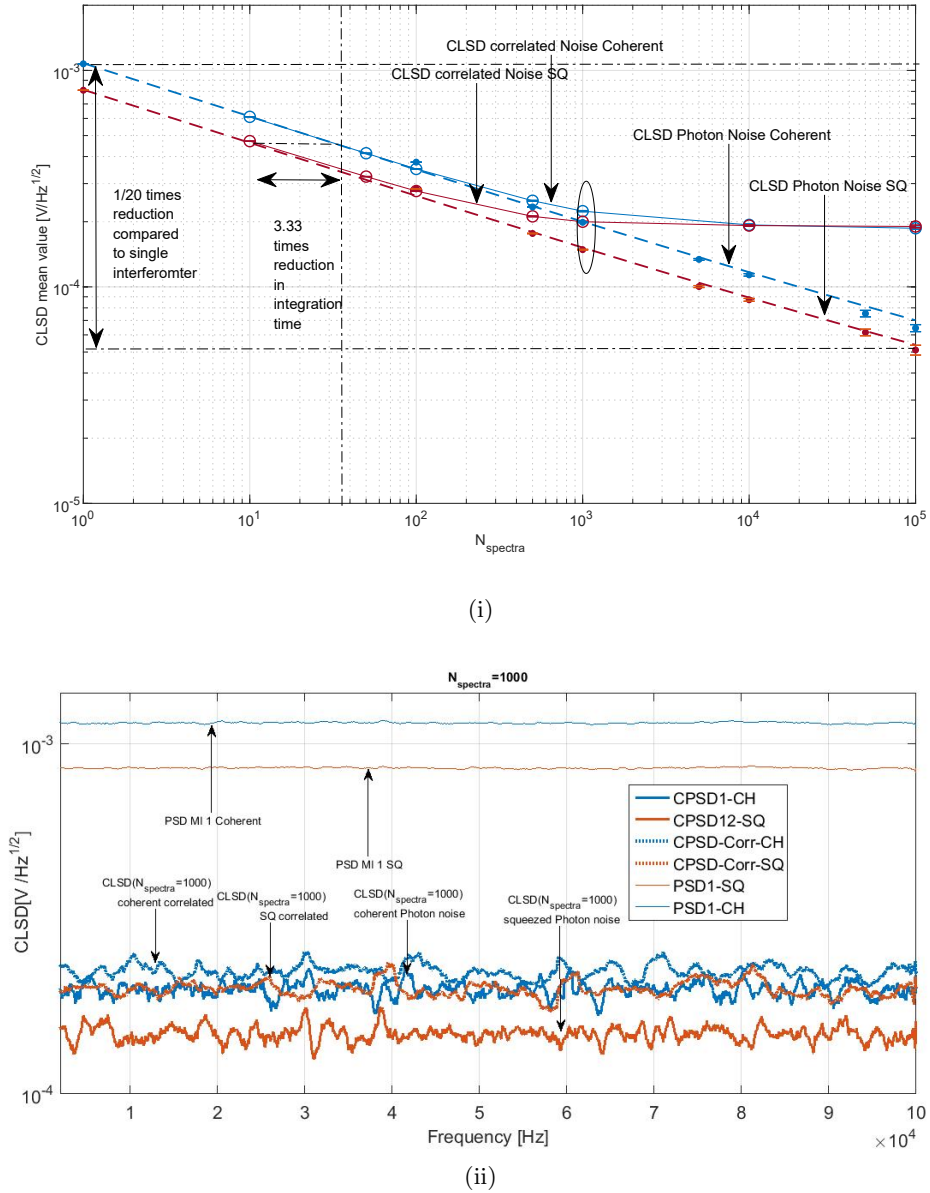
Figure 5.10: (i)The figure above presents the Cross linear Spectral density as a function of Number of Spectra. It can be seen that for low values of N_{\text{spectra}} it scales as N_{\text{spectra}}^{-1/4} while for higher values of N_{\text{spectra}} it reaches a plateau. (ii) The figure above corresponds to the CLSD evaluated at N_{\text{spectra}} = 1000 and PSDs of the first interferometer.
