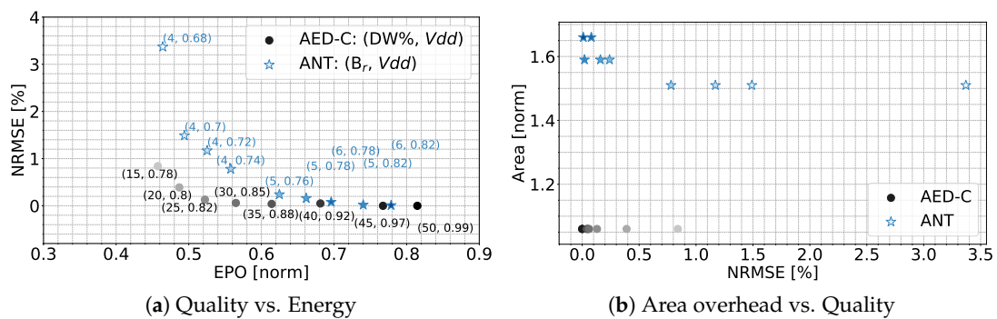
Figure 12. ANT vs. AED-C timing speculation: FIR filter.
