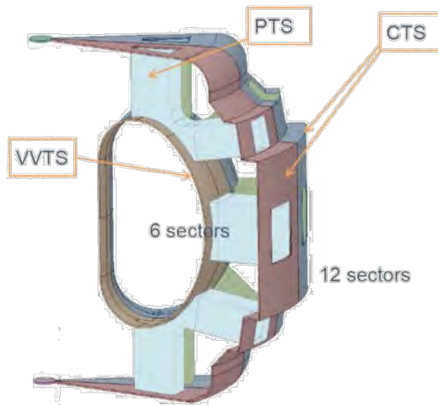
Figure IV.27: Schematic view of the DTT thermal shield
