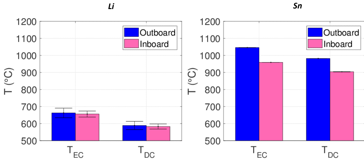
Figure III.21: Temperatures of the LM-vapour system within the various chambers for Li (left) and Sn (right). Error bars account for uncertainty on the particle dwell time of impurities in the plasma, \tau (very small effect for Sn).
