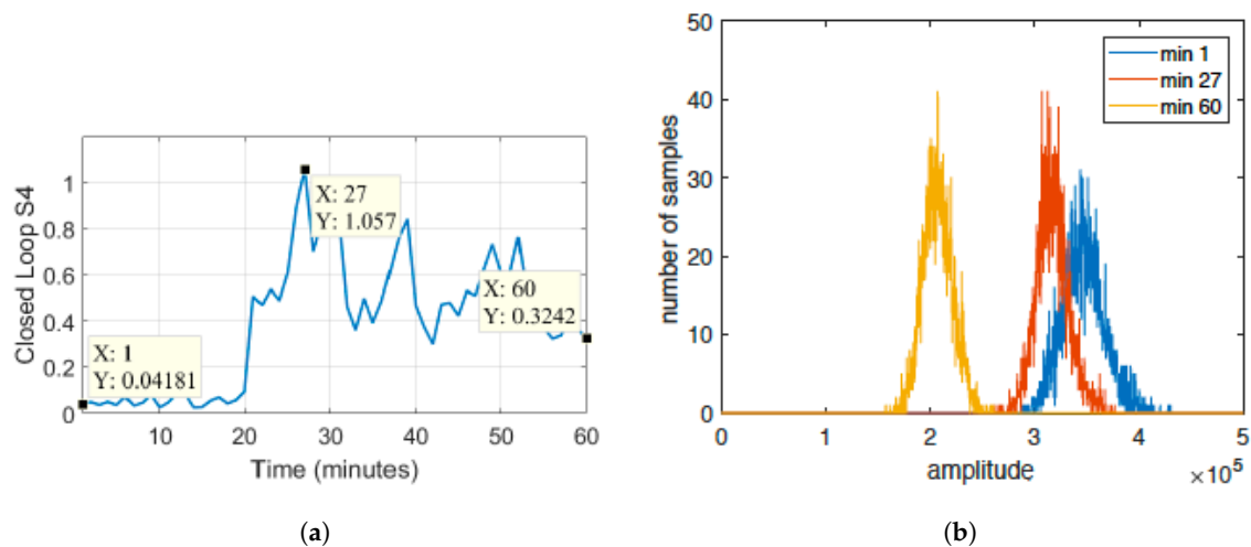
Figure 1. The distribution of the signal samples varies according to scintillation intensity; (a) values of the amplitude scintillation index S_4 over time; (b) histogram of the Signal Intensity (SI) for three different values of amplitude scintillation taken at three different time instants.
