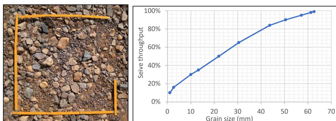
Figure 8. Representative grain size distribution of sediments along the Sirba River.
