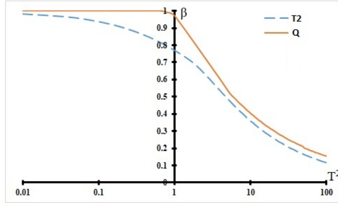
Fig. 4. The exact phase-locking domain for the system (39) vs. its estimate from Theorem 2.
