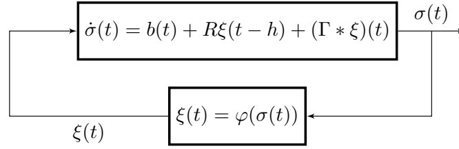
Fig. 1. The system (1) as a feedback interconnection of two subsystems
