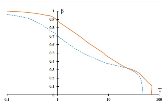
Fig. 6. Stability domains for the PLL system with time delay (42).
