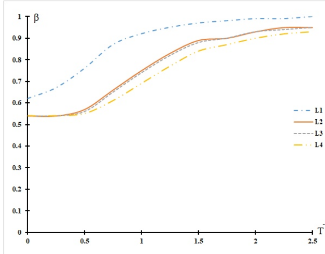
Fig. 5. Stability domains for the PLL system (41) with m = 0.2 .
