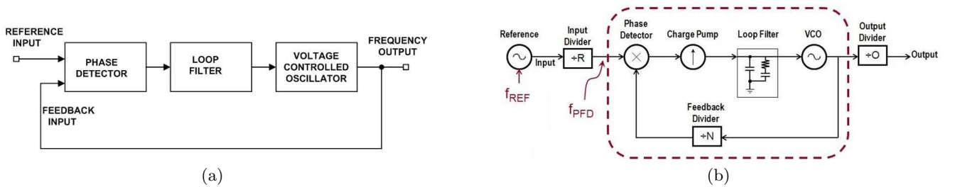
Fig. 3. Illustration to Subsection 2.2.3: the “minimal” PLL vs. a more general synchronization circuit
