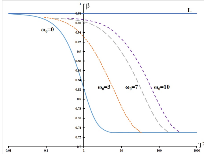
Fig. 8. Domains of stability and slow oscillations for the system (41) with m = 0.4 .
