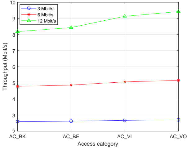
Figure 4: Measured throughput with a single stream, at different ACs and physical data rates; payload length: 1470 B, offered traffic: 10 Mbit/s
