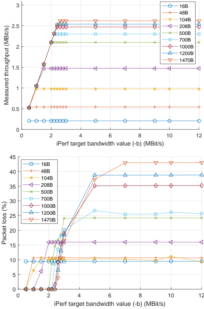
Figure 1: Throughput (top) and Packet loss (bottom) measurements for 3 Mbit/s of physical layer data rate, with different payload size and offered traffic values
