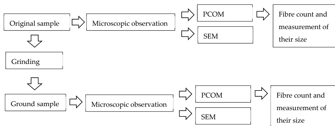
Figure 3. Analysis procedure flowsheet.
