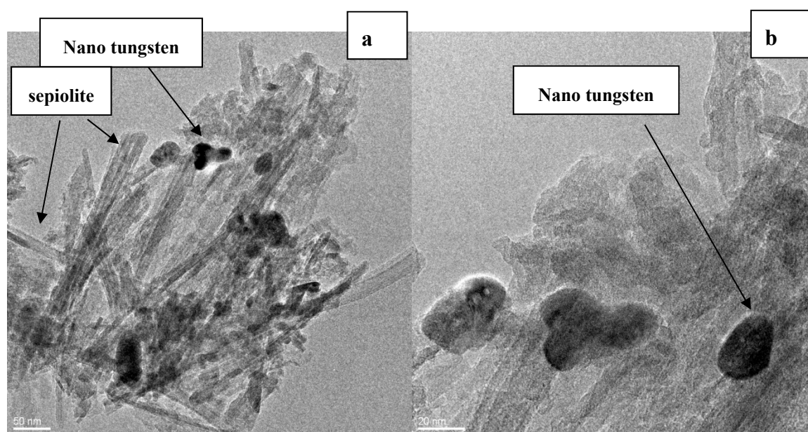
Figure 3. HRTEM of tungsten-modified sepiolite: (a) low and (b) high magnification.
