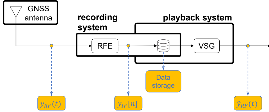
Figure 6.1: R&R system for GNSS signals. Block scheme.
