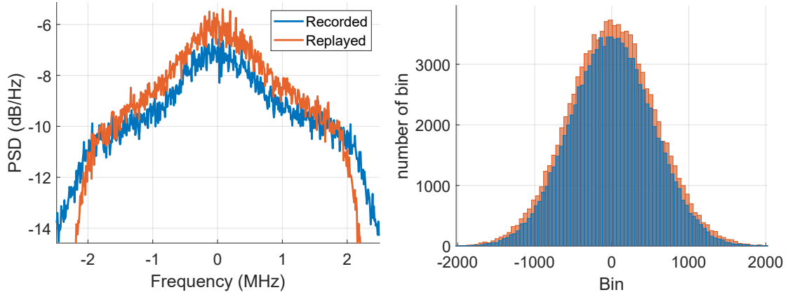
Figure 6.4: PSD (left) and histogram (right) of the recorded (blue) and replayed (orange) signals.
