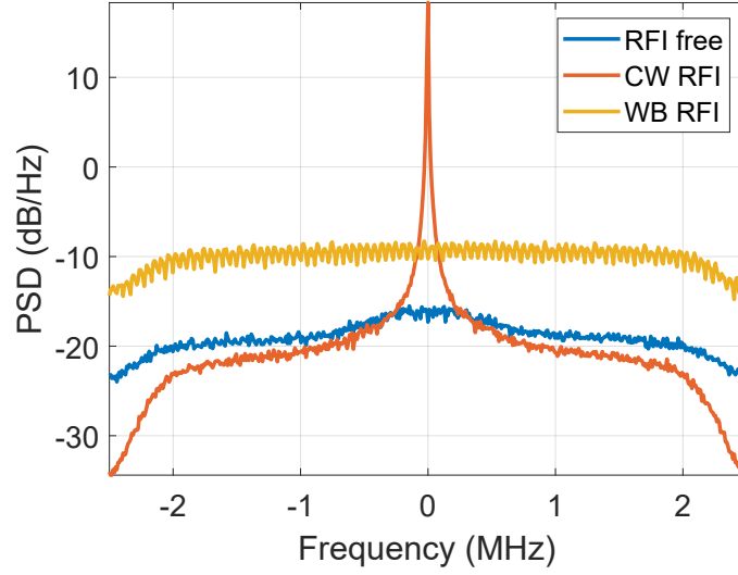
Figure 6.18: Estimation of PSD for different interfering signals.
