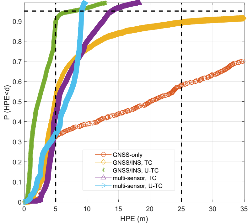
Figure 9.2: CDFs for CaseB .
