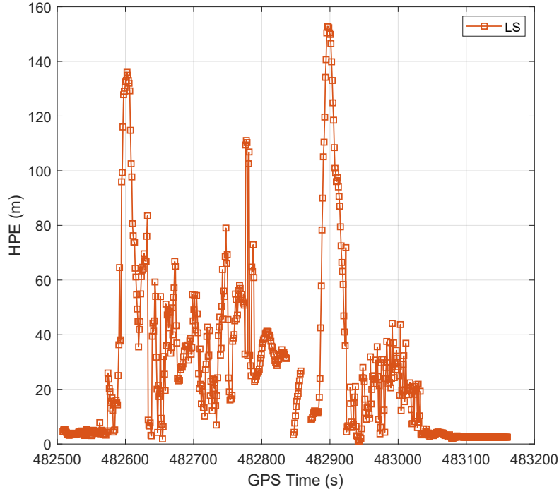
Figure 7.12: GNSS standalone results (orange) for CaseB and reference trajectory (blue). HPE over time.
