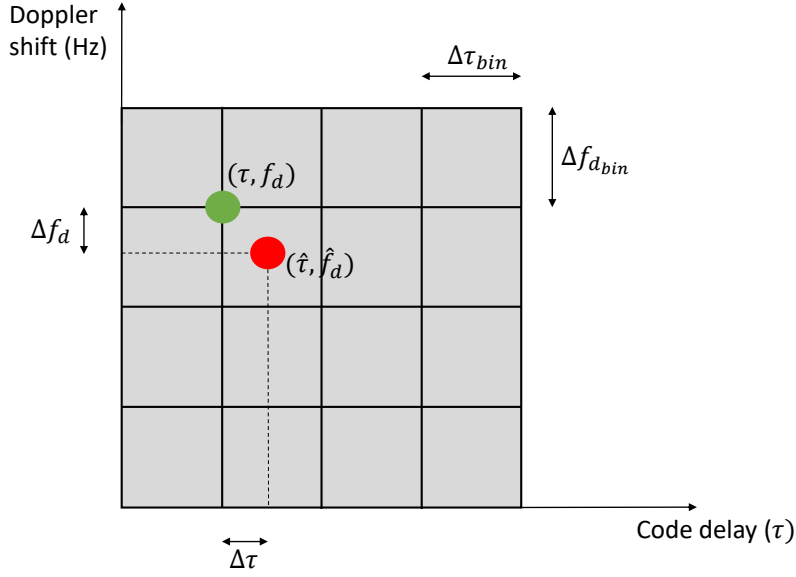
Figure 3.2: Example of search space.
