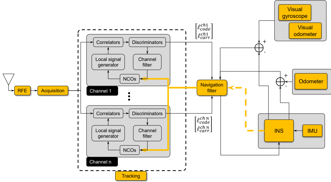
Figure 5.4: Architecture of a multi-sensor GNSS receiver U-TC with INS, visual sensor and odometer.
