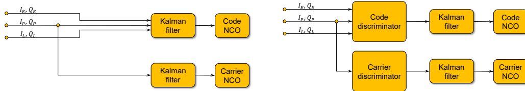
Figure 3.8: Coherent (left) and non-coherent (right) KF-based tracking.
