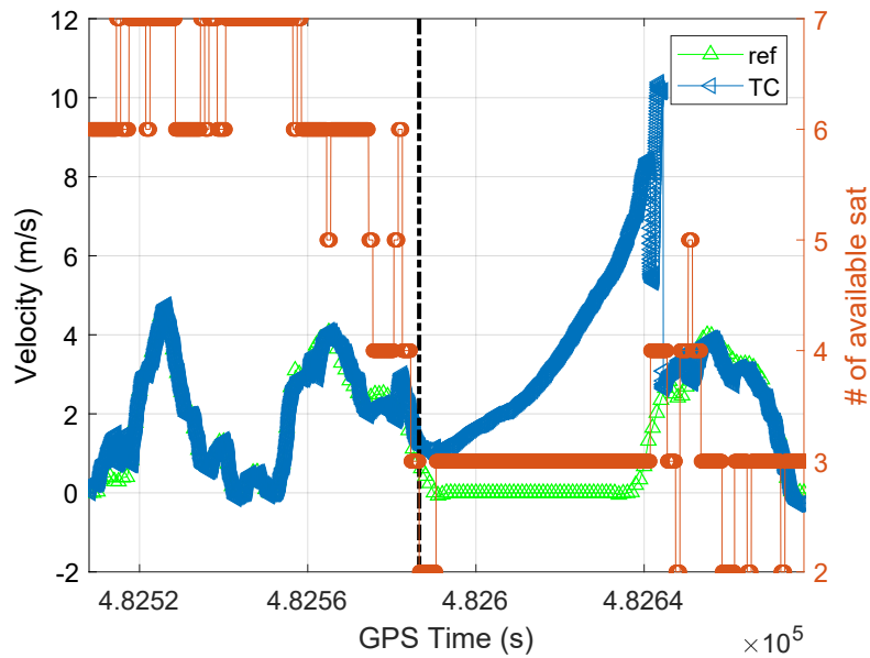
Figure 7.17: CaseB . Zoom to the point where the TC started drifting. Velocity estimated by the reference system (green) and by the TC (blue). Number of available satellites (orange).
