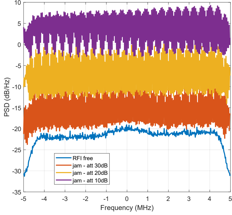
Figure 8.4: Estimation of PSD for different jamming signal strengths.
