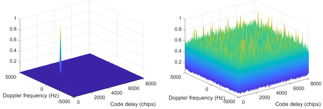
Figure 3.3: Example of CAF over the search space evaluated on a Galileo PRN12 (left) and for PRN21 (right) realistic signal.
