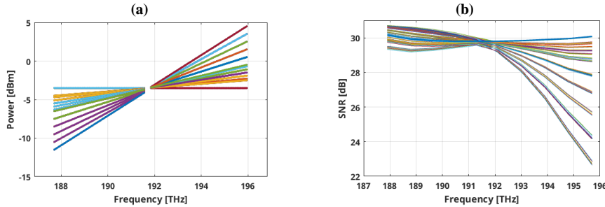
Fig. 3: Tilting strategies as at the span inlets (a) and the corresponding SNR curves after one span propagation (b)
