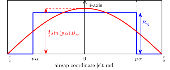
Fig. 2. Shape of the airgap flux density generated by the PMs on one pole pitch (blue) and its first harmonic (red).
