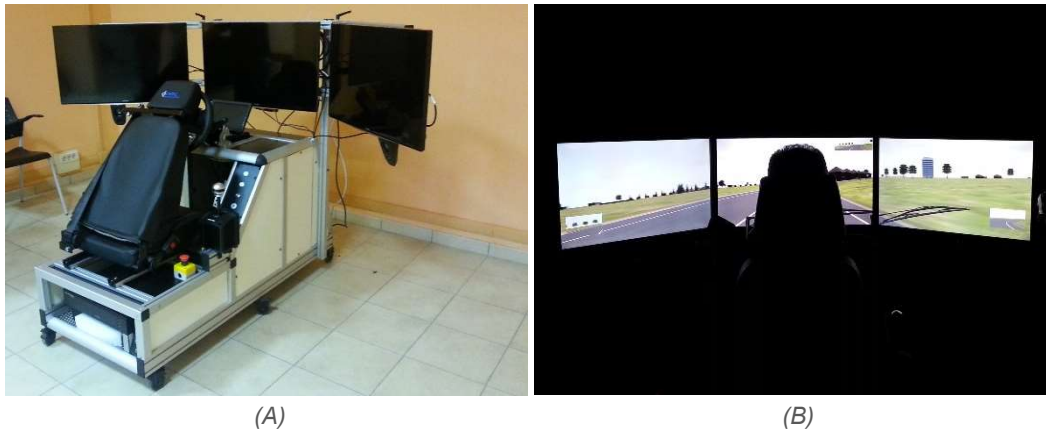
Figure 2.1. (A) First picture of the driving simulator in the Road Safety and Driving Simulation Laboratory; (B) picture of a simulation in the new dark room
