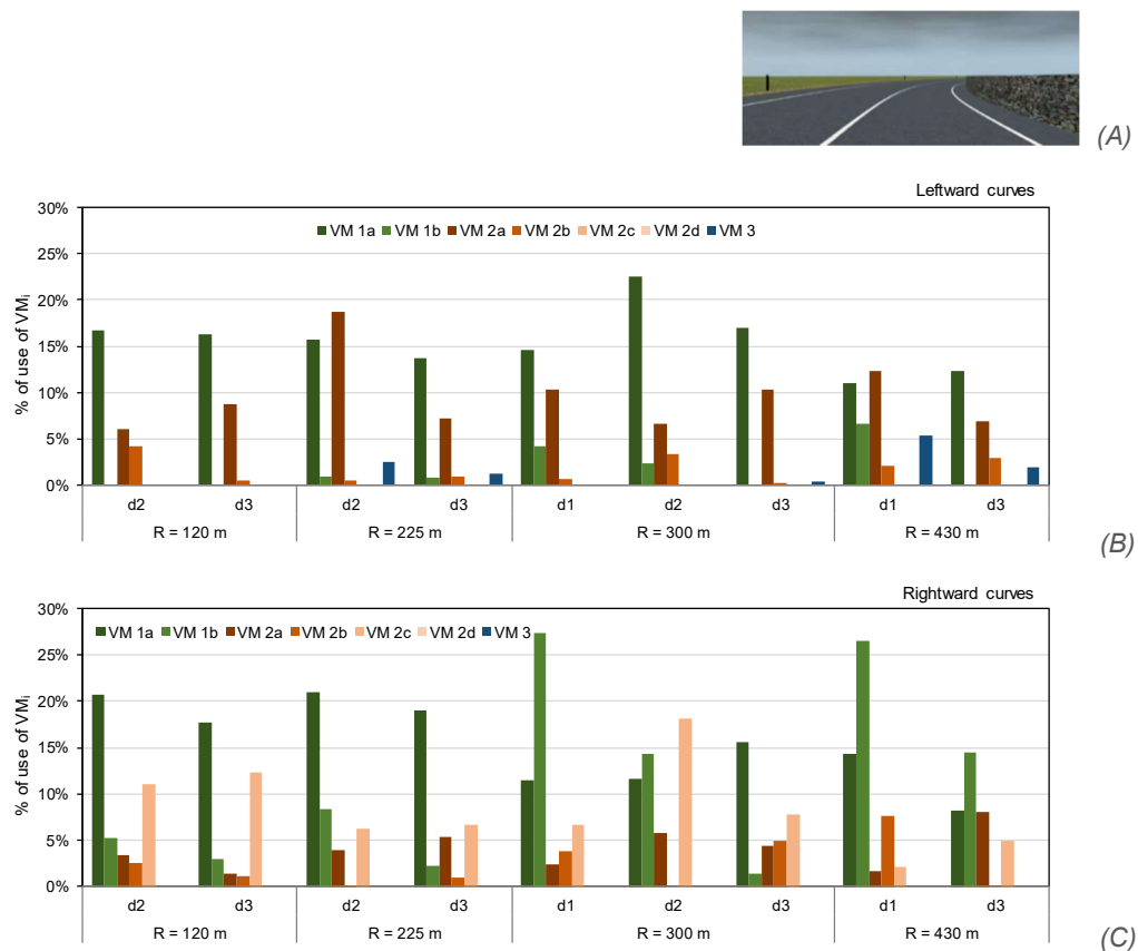
Figure 8.25. (A) Picture of the virtual scenario; in the graphs, the percentage of use of VMs for the Combination #7 along (B) leftward and (C) rightward curves ( d1 = 0 m; d2 = 1.5 m; d3 = 3 m)
